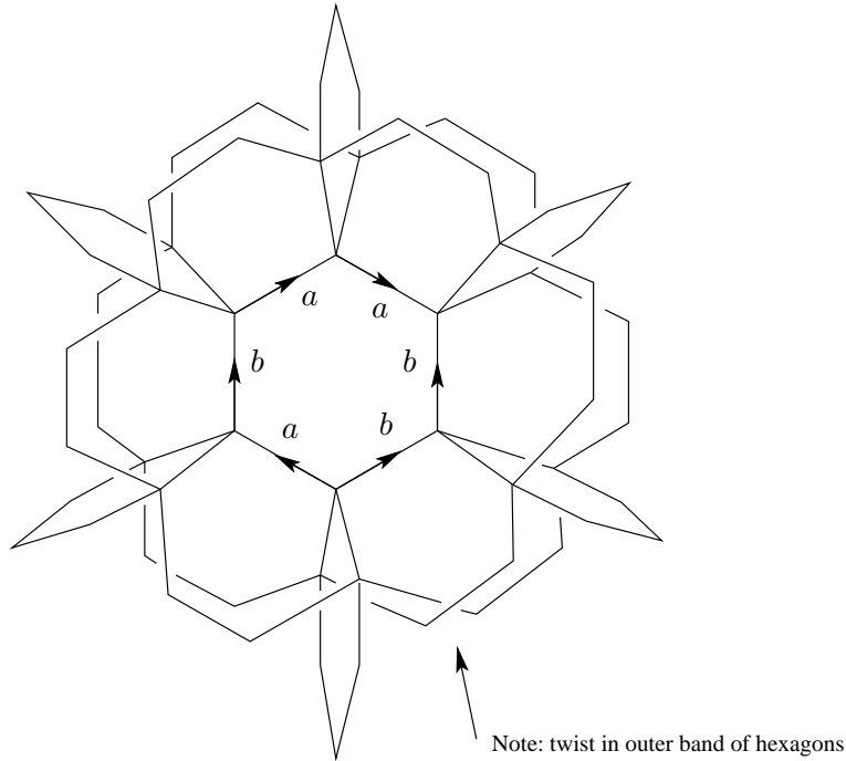
FIGURE 3. The Cayley complex for \langle a, b \mid aba^2 = b^2 \rangle .
