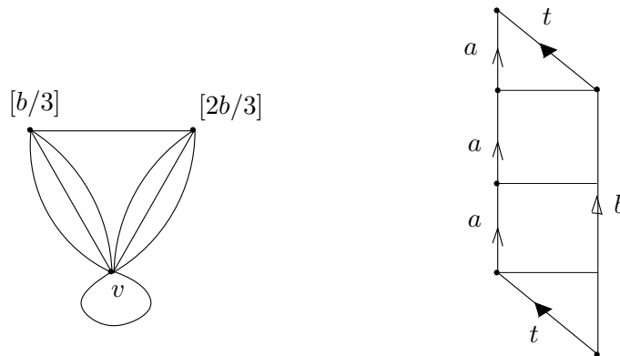
FIGURE 5. The Morse function on the extra 2-cell in the F_6 \rtimes \mathbb{Z} group, and the level set through v .
